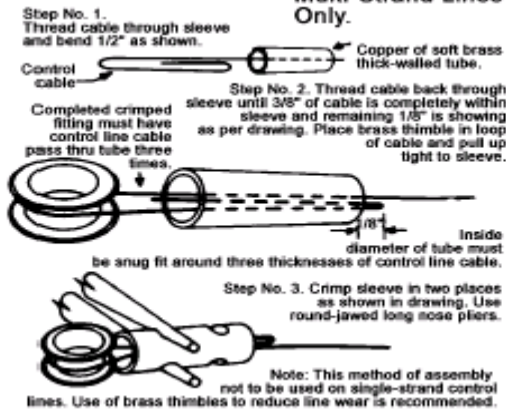
Figure 4. Alternate Construction Multi-Strand Lines Only.
