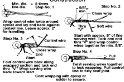
Figure 4. Alternate Construction Multi-Strand Lines Only.
