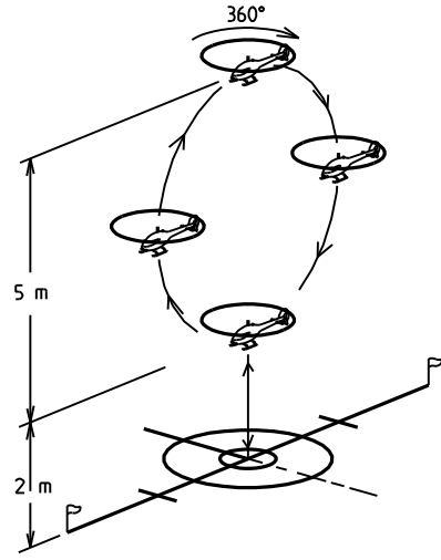
19.3.2 Circle with 360° Pirouette
